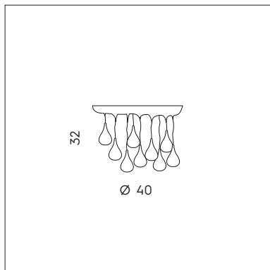
LS 1045/40P 30W LED 3500 lumen 3000K CE
