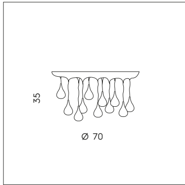
LS 1045/70P 30W LED 3500 lumen 3000K CE
