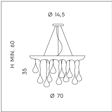
SP 1045/70S 30W LED 3500 lumen 3000K CE
